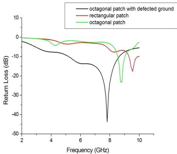
Fig. 2: Return loss of the proposed antenna.
