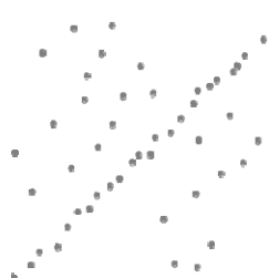
A data set with many outliers for which a line has to be fitted.
